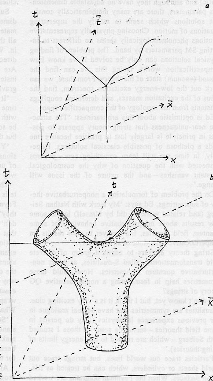
Figure 4. Contact interactions for particles and strings. a , Interactions between particles occur at a single spacetime point, called the vertex in the Feynman diagram approach. This point is Lorentz-invariant since it is the same in all reference frames. b , The splitting of a closed string into two closed strings, otherwise known as the pants diagram. The world surface is a cylinder, so the interaction region is no longer a point. One observer will see the interaction occur at point (1), and another will see it occur at (2). The contact point is no longer Lorentz-invariant. Divergences in QFTs of point particles can arise when two sharp vertices get arbitrarily close to one another. Renormalization is needed to remove the ultraviolet divergences by introducing ultraviolet momentum cutoffs, thereby 'fuzzifying' out the vertices. Since string diagrams are surfaces, they tend to accomplish this process automatically. See Quantum Field Theory of Point Particles and Strings , B. Hatfield, Addison-Wesley, 1992.
