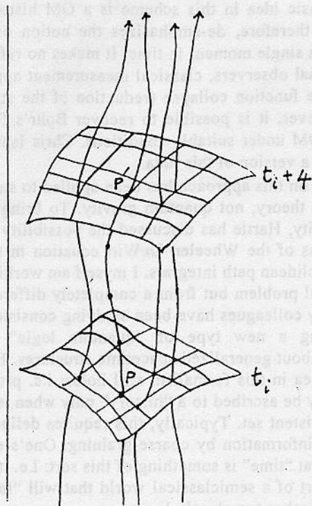
Figure 1. Foliating spacetime into a one-parameter family of space-like hypersurfaces: In Newtonian mechanics, a given moment of time has the same meaning for all observers. Time is absolute. In SR, this notion is somewhat ambiguous because of the nonuniversality of simultaneity. However, once an inertial frame is specified, the notion becomes more precise. Unless spacetime is flat, there are no global inertial frames in GR. So 'a moment of time' in GR is ambiguous. However, a more general concept replaces it; the notion of 'a given space-like hypersurface'. It is possible to 'slice up' or foliate spacetime into a one-parameter family of 3D space-like surfaces, filling out all of spacetime. At each event on a surface, there is a local Lorentz frame whose surface of simultaneity coincides locally with the hypersurface. Lorentz frames at various events do not mesh to form a global inertial frame, but their simultaneity surfaces mesh to form the actual space-like hypersurface. This is a picture of two space-like hypersurfaces through events P and P' which occur at different times. World lines of observers cross these surfaces orthogonally, and are labelled by (x_1, x_2, x_3) , x_0 = t_i + \tau , where \tau is the proper time measured along the worldline. Note that the third coordinate x_3 is suppressed in the diagram. Arbitrary coordinate grids defining x_1 and x_2 are drawn on the hypersurfaces. At the point of crossing a hypersurface, the proper time (defined by an observer's wristwatch) reads the same as other observers' watches. Such a surface defines a notion of 'simultaneity'. Another surface of simultaneity through the event P may have a different slope or curvature (defining different local Lorentz frame). This second surface is defined by another set of observers with their own wristwatches, and their own proper time readings. It is also possible to push the hypersurface ahead in time at different rates in different places, so long as the hypersurface stays spacelike. This idea of a 'many-fingered' time is GR's dramatic new contribution to our understanding of time. See, for example, Gravitation , C. Misner, K. Thorne and J. Wheeler, W.H. Freeman and Co., 1973.
